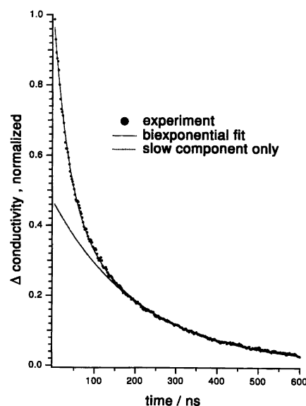
Fig. 4. Production of HMI in cyclohexane by two-photon laser excitation of triphenylene radical cations. 22 Dots: increment in the dc conductivity caused by 532 nm (2.3 eV), 40 mJ pulse from an Nd:YAG laser applied 270 ns after 248 nm (5 eV), 10 mJ pulse from a KrF excimer laser. Solid curve: biexponential fit with \tau_{\text{fast}} = 32 \text{ ns} and \tau_{\text{slow}} = 210 \text{ ns} . The dashed curve is the slow component.
