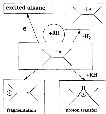
Fig. 1. Reaction scheme for radical cations.
