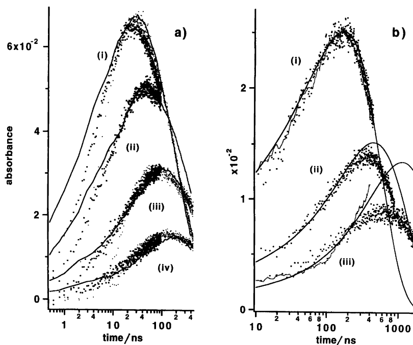
Fig. 6. Formation of perylene radical cation in the pulse radiolysis of decalin solutions, from Ref. 17. Formation of perylene •+ in N 2 O-saturated decalin solution (63 cis -: 37 trans -decalin mixture) with (a) no and (b) 0.1 mol dm -3 toluene. Concentrations of perylene are given in the units of 10 -4 mol dm -3 : for (a) (i) 5.5 (ii) 2.8 (iii) 1.25 (iv) 0.44; for (b) (i) 5.7 (ii) 2.5 (iii) 1.1. Short timescale kinetics in (a) ( solid dots ) were obtained with 30 ps electron pulses, all other kinetics were obtained with 4 ns pulses (6–8 krad pulse -1 ). Solid lines in (a) are a Monte-Carlo simulation for an HMI that lives 150 ns. Solid lines in (b) represent a simulation using the continuum-diffusion model (compare with the broken curves calculated with the Monte-Carlo model). The discrepancy at t > 0.5 \mu\text{s} is due to homogeneous recombination, which was not included in the calculation.
