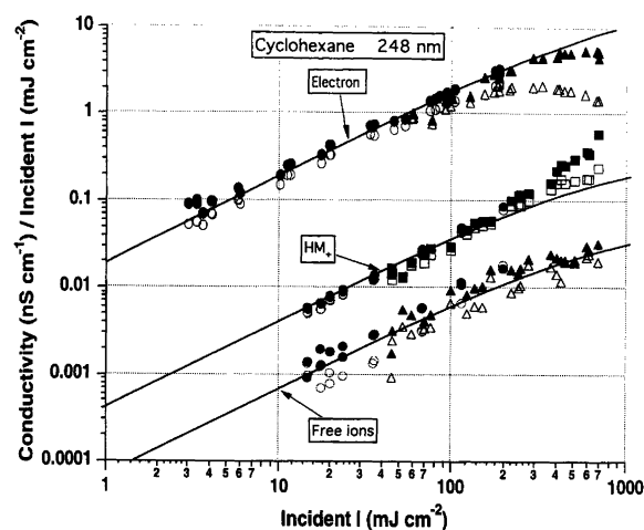
Fig. 3. An example of photon flux dependence studied by transient dc conductivity. Intensity dependence of ionization in cyclohexane at 248 nm (5 eV). The upper trace is for Ar-saturated solution and the middle and lowest traces are for \text{SF}_6 -saturated solutions. For the upper traces the signal is mainly from solvated electrons, with a negligible contribution from cations; the middle set is the signal from HMI (the free ion signal at 2 \mu\text{s} has been subtracted). For the upper and middle traces, the open symbols represent the observed signals at 50 ns after the laser pulse, and the filled symbols represent these signals corrected for second-order neutralization, which becomes appreciable at the higher light intensities. The circles are for runs where the cross-sectional area of the laser beam was 0.3 \text{cm}^2 ; the squares and triangles are for runs where the area was 0.14 \text{cm}^2 . Data for the free ions (lowest traces) were obtained by a fitting procedure (open symbols) and measurement at 2 \mu\text{s} (filled symbols). The curves are calculated as described in Ref. 18 for a two-photon ionization process.
