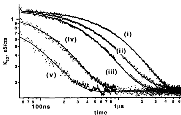
Fig. 5. Pseudo-first-order scavenging of HMI in decalin. 15 Scavenging kinetics of HMI in \text{CO}_2 -saturated decalin mixture (1:3 trans/cis decalin). Dots: decay kinetics of transient dc conductivity in 248 nm laser photolysis of the decalin mixture containing (i) no, (ii) 10^{-5} , (iii) 2 \times 10^{-5} , (iv) 10^{-4} , and (v) 2 \times 10^{-4} \text{ mol dm}^{-3} cyclohexene. Solid lines: best-fit kinetics obtained using a model of a single HMI.
